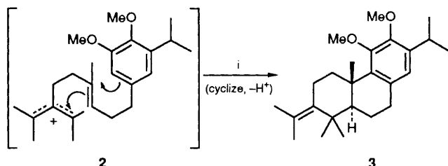
Scheme 1 Reagents and conditions: i, 0.5% \text{CF}_3\text{CO}_2\text{H-CH}_2\text{Cl}_2 , -45^\circ\text{C}
