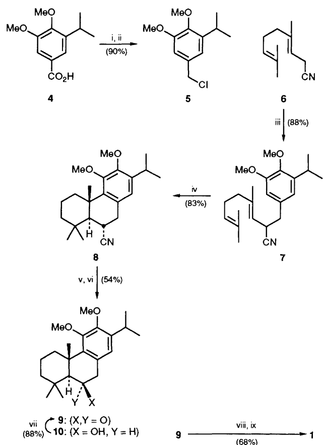
Scheme 2 Reagents and conditions: i, BMS, THF; ii, \text{SOCl}_2 , \text{CH}_2\text{Cl}_2 ; iii, (a) LDA, THF, (b) 5 ; iv, \text{BF}_3 , \text{MeNO}_2 ; v, (a) LDA, THF, (b) \text{O}_2 , (c) \text{SnCl}_2 , \text{HCl} (aq.); vi, \text{LiAlH}_4 , THF; vii, PDC, \text{CH}_2\text{Cl}_2 ; viii, \text{BBR}_3 , \text{CH}_2\text{Cl}_2 ; ix, \text{O}_2 , silica gel
